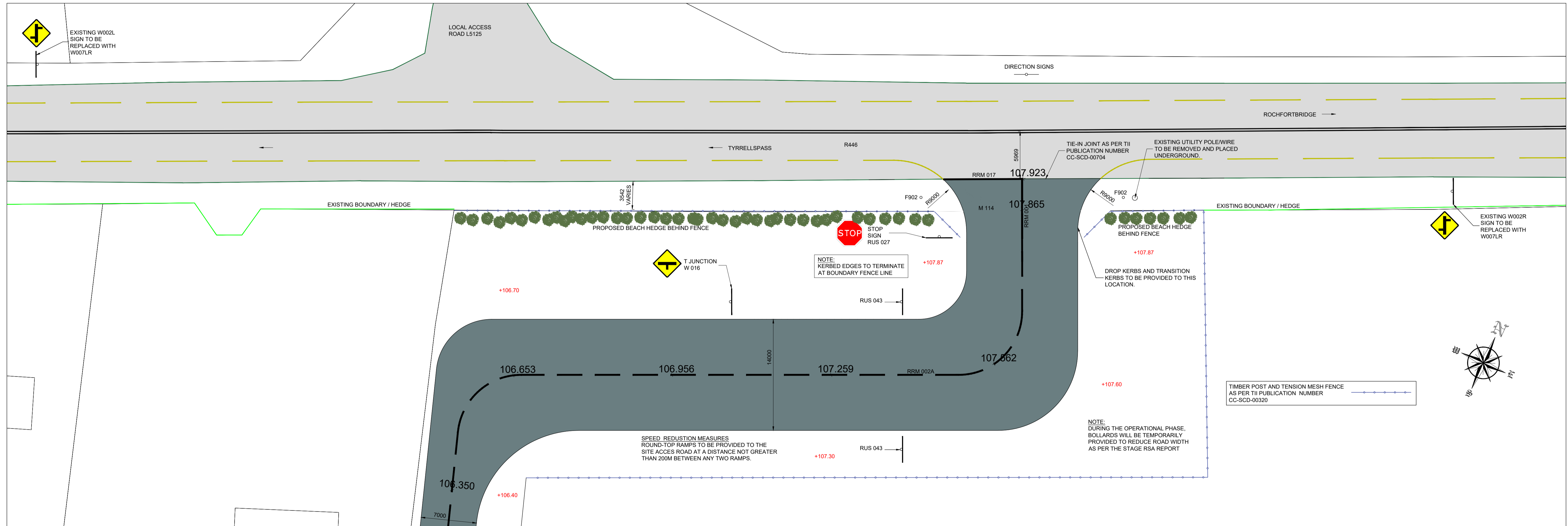
JUNCTION ROAD MARKINGS SCALE 1:250
