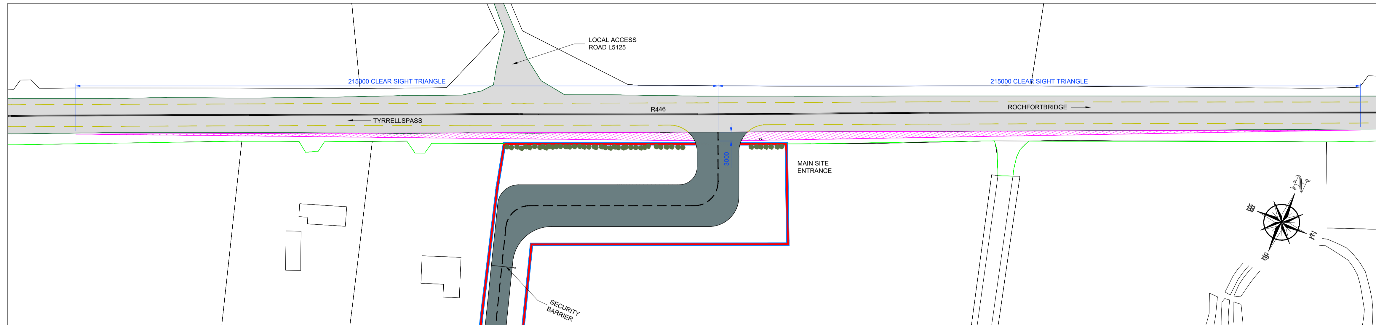
JUNCTION SIGHT LINES SCALE 1:750
